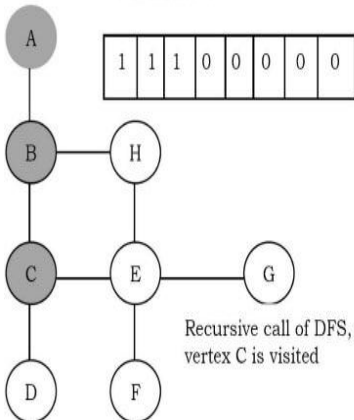
Visited Table
