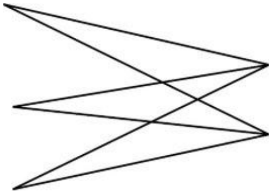
K_{2,3}
